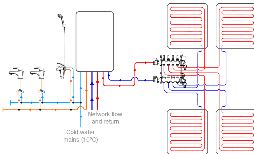
Fig 7 – example HIU with underfloor heating manifold
